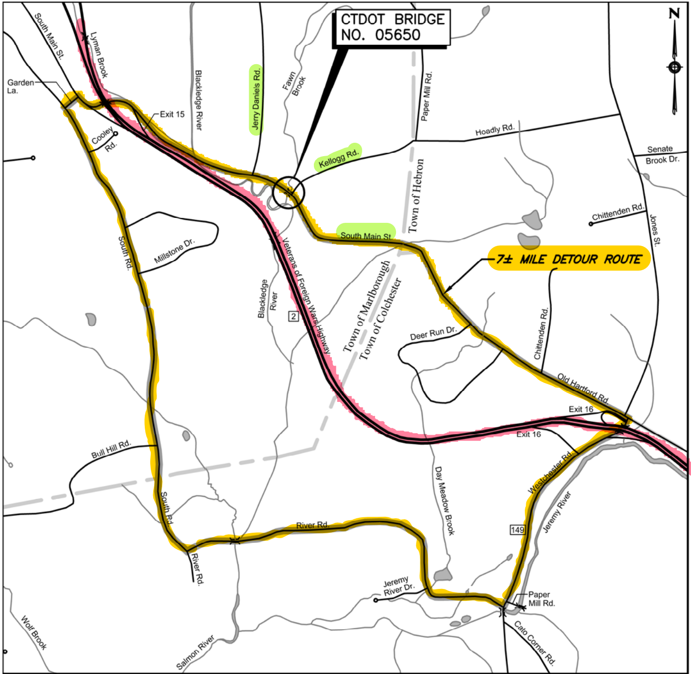
TEMPORARY CONSTRUCTION DETOUR PLAN
